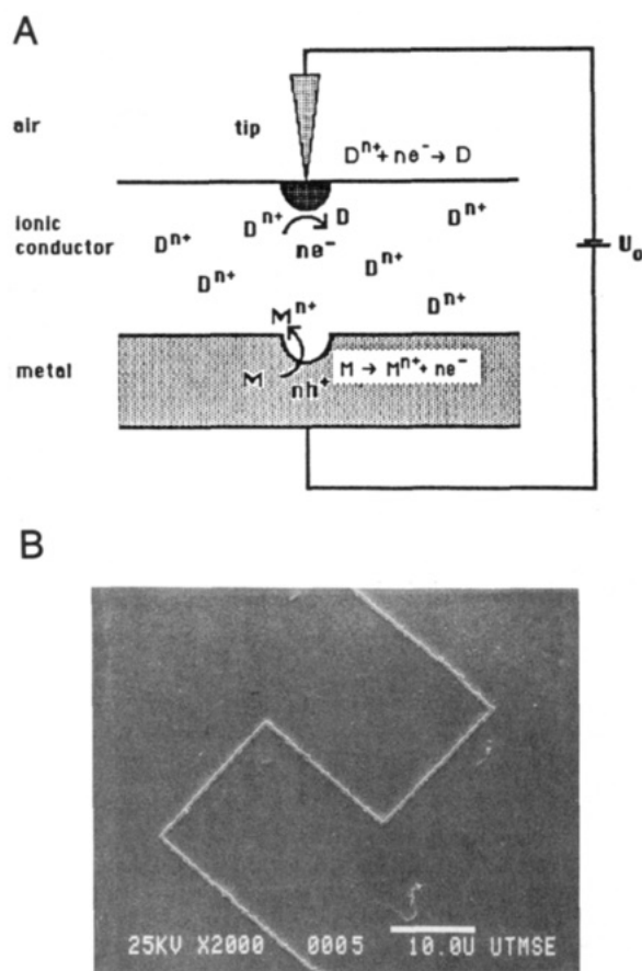
Figure 6. (A) Schematic representation of the SECM operating in the direct mode. (B) Scanning electron micrograph of silver lines deposited in a Nafion film by using the SECM in the direct mode. Tip material, tungsten; bias, 5 V; tip current, 0.5 nA; and scan rate, 900 Å/s. 23 Reprinted with permission from ref 23. Copyright 1989 The Electrochemical Society, Inc.
