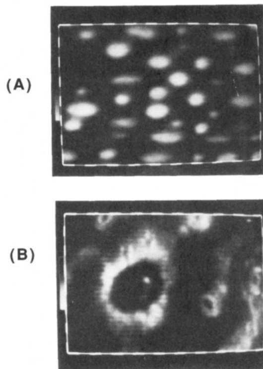
Figure 5. Gray-scale image of biological substrates in a 20 mM \text{K}_4\text{Fe}(\text{CN})_6 and 0.1 M KCl solution scanned with 1- \mu\text{m} -radius Pt tip: scan area, 188 \times 142 \mu\text{m} (white lines around edge: 10 \mu\text{m} ). (A) Top surface of grass. (B) Bottom surface of L. sinense leaf.
