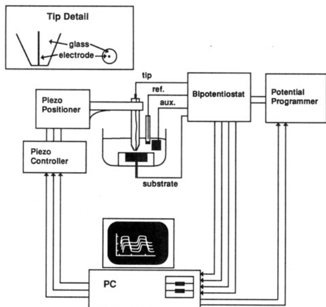
Figure 1. Block diagram of the SECM apparatus.
