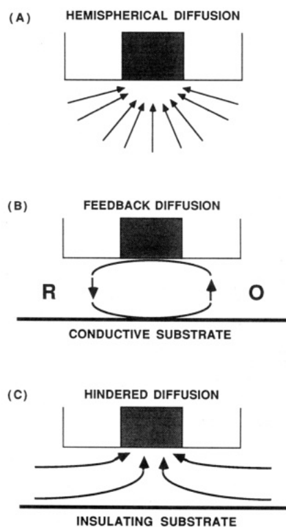
Figure 2. Basic principles of scanning electrochemical microscopy (SECM): (A) far from the substrate, diffusion leads to a steady-state current, i_{T,\infty} ; (B) near a conductive substrate, feedback diffusion leads to i_T > i_{T,\infty} ; (C) near an insulating substrate, hindered diffusion leads to i_T < i_{T,\infty} .
