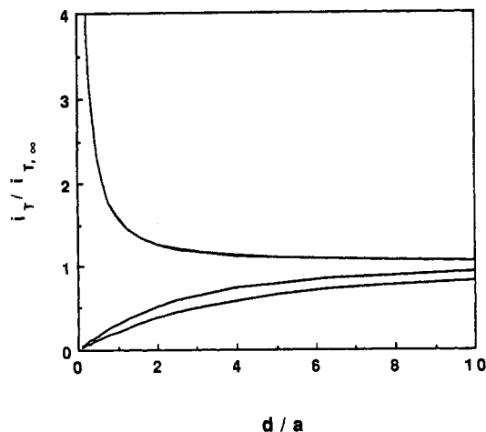
Figure 3. Plot of i_T normalized with respect to i_{T,\infty} as a function of the tip-substrate distance normalized with respect to the radius a of the tip. Above a conducting substrate (top curve), different sheath sizes exhibit no difference in tip current. Above an insulating substrate (bottom curves), different sheath sizes lead to different tip currents (the larger the sheath, the smaller the tip current).
