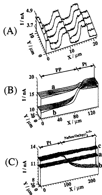
Figure 4. (A) Scan of an IDA: tip, 0.1- \mu\text{m} -radius Pt microdisk electrode; E_T = -0.78 V vs SCE; solution, 0.2 M MVCl 2 and 2 M KCl; |i_{T,\infty}| = 3.7 nA. (B) Scans of the boundary between PP and Pt ( d = 6 \mu\text{m} ): tip, 5.5- \mu\text{m} -radius C microdisk electrode; E_T = -0.4 V vs SCE; solution, aqueous 10 mM Ru(NH 3 ) 6 Cl 3 and 0.1 M K 2 SO 4 ; |i_{T,\infty}| = 12.5 and 13.5 nA for planes a and b, respectively. Plane a, at E_S = 0.7 V (PP: conductor); plane b, at E_S = -0.1 V (PP: insulator). (C) Scans of the boundary between Pt and a Nafion film containing Os(pbpy) 3 2+ in a 10 mM K 3 Fe(CN) 6 and 0.1 M Na 2 SO 4 solution; tip, 5.5- \mu\text{m} -radius C; E_T = -0.4 V vs SCE. (a) i_{T,\infty} plane at d = 98 \mu\text{m} ; (b) at E_S = 0.42 V [Os(pbpy) 3 2+ form] and d = 10 \mu\text{m} ; (c) at E_S = 0.8 V [Os(pbpy) 3 3+ form] and d = 10 \mu\text{m} .
