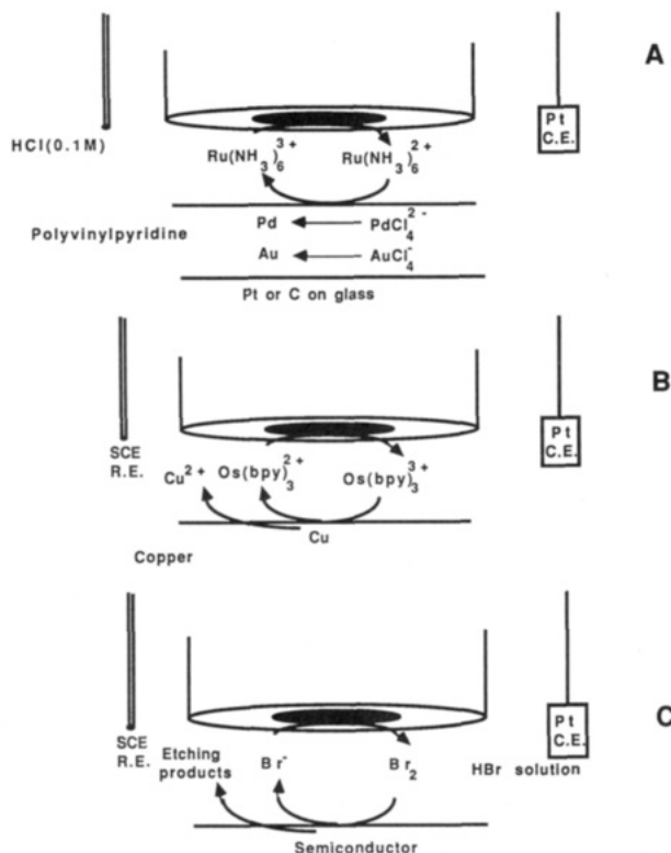
Figure 7. Schematic representation of the SECM applied in the feedback mode for (A) metal deposition, (B) copper etching, and (C) semiconductor etching.
